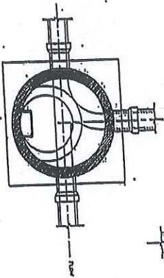
TYPICAL MANHOLE BEDDING
